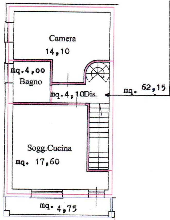
PIANO TERRA
