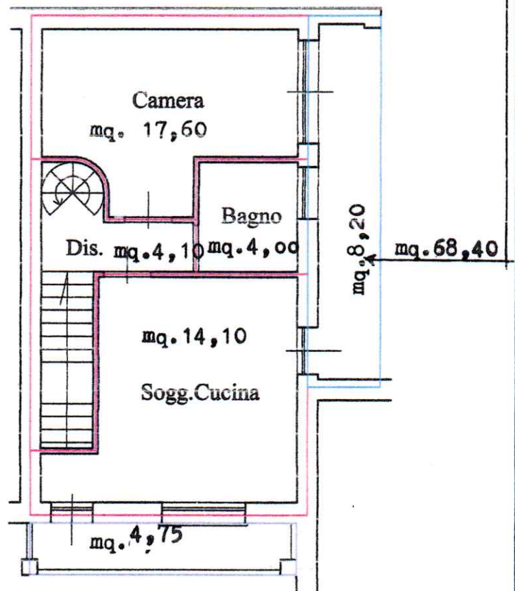
PIANO TERRA
